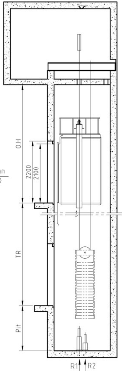
Shaft vertical section
