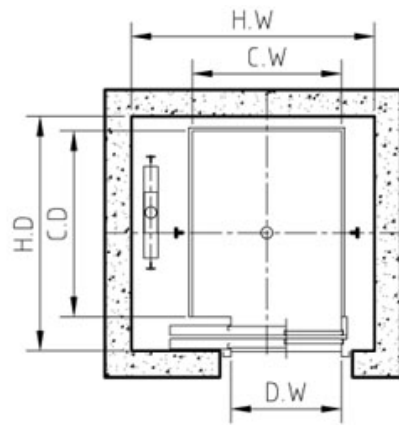
Shaft plane layout
