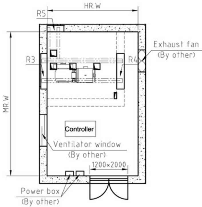
Machine room plane layout
